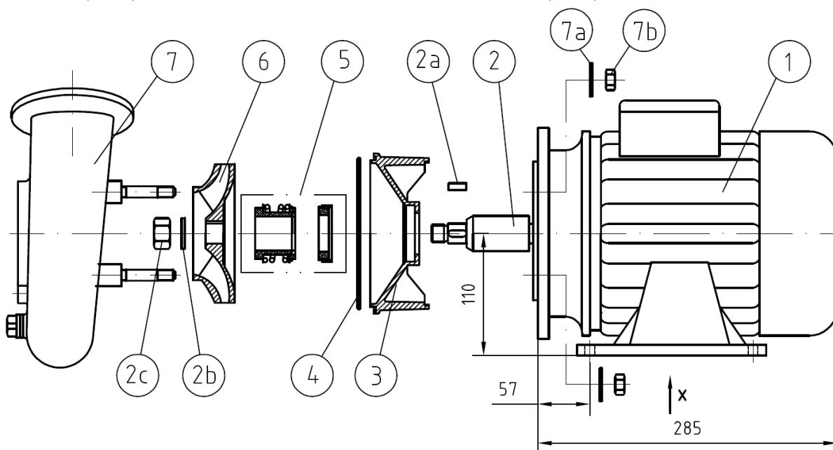
2,2kW, 230V FB65 Art.7752150
